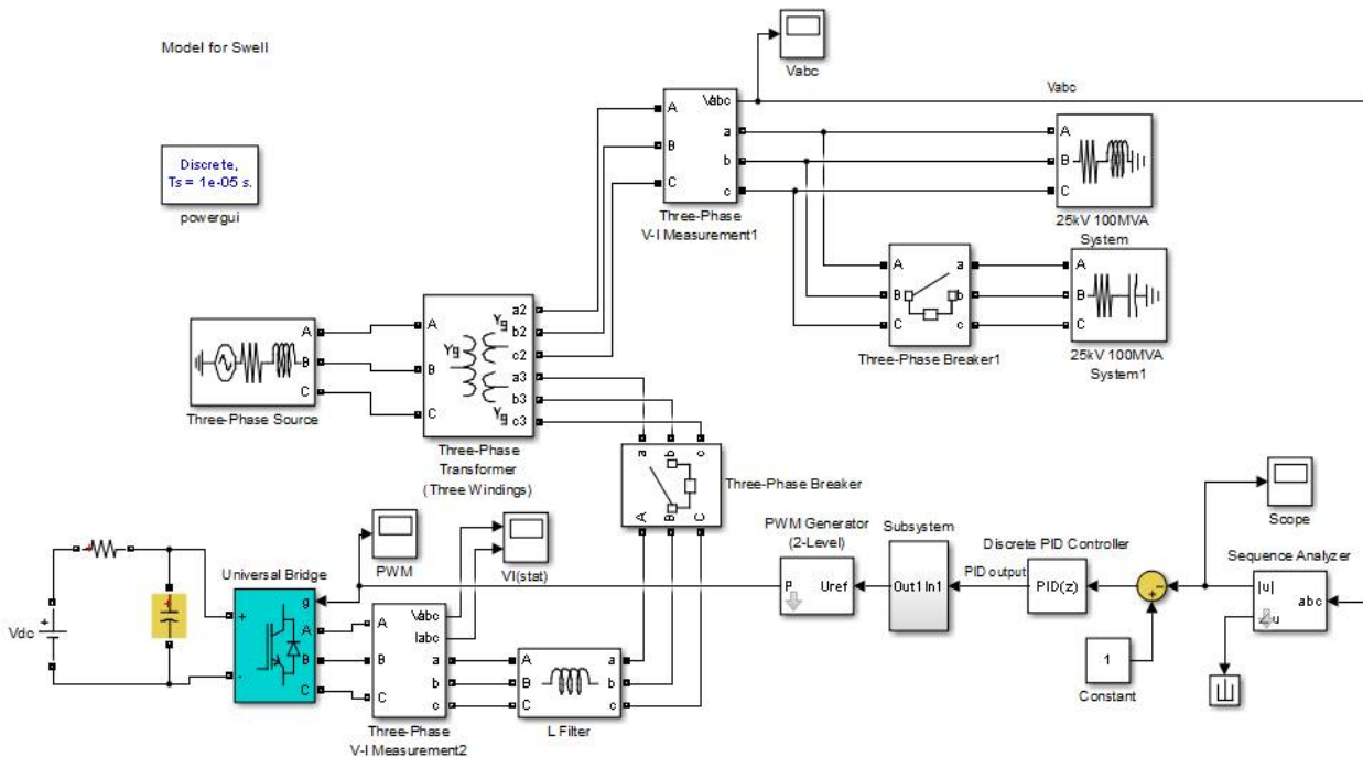
Fig. 5 simulation model for swell
