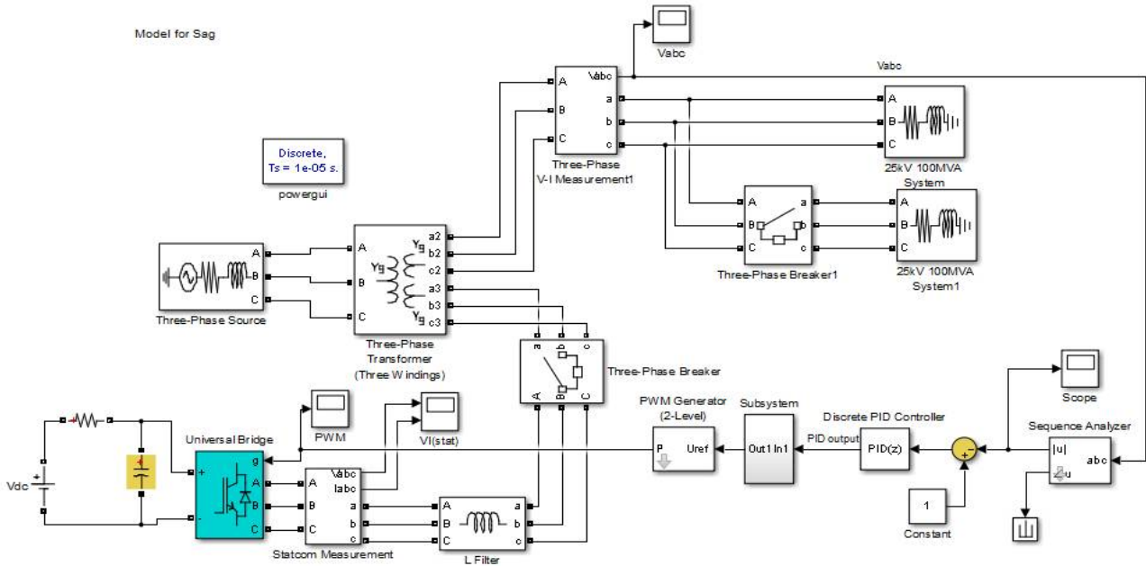
Fig. 4 simulation model for sag
