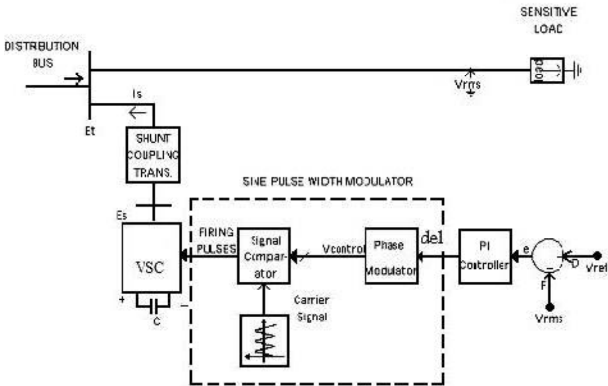
Fig 1. Control scheme designed for the D-STATCOM
