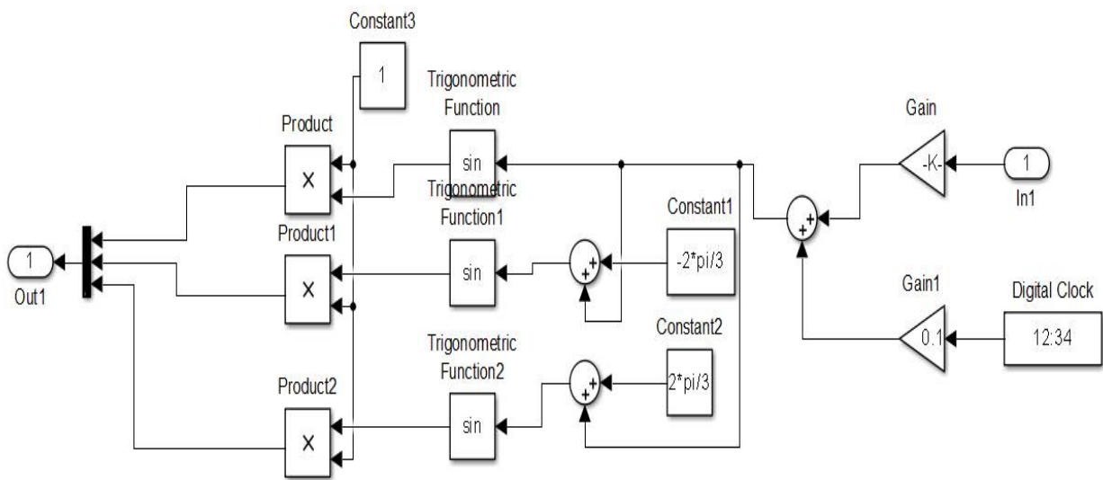
Fig 6 phase modulation of the control angle \delta
