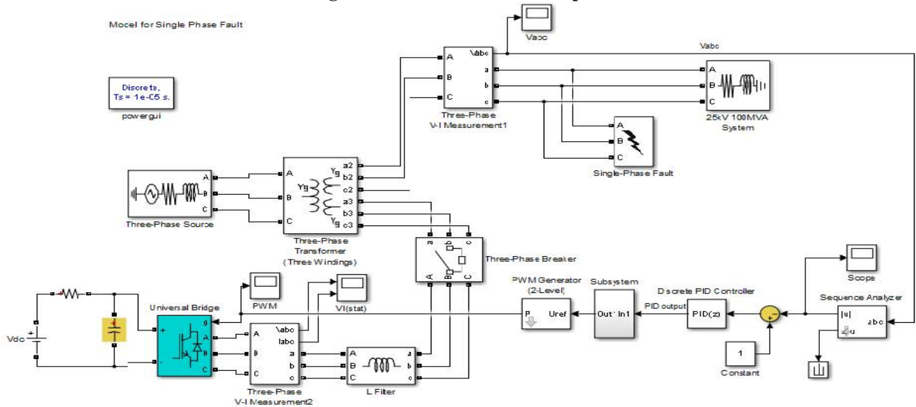
Fig. 3 simulation model for the single phase fault
