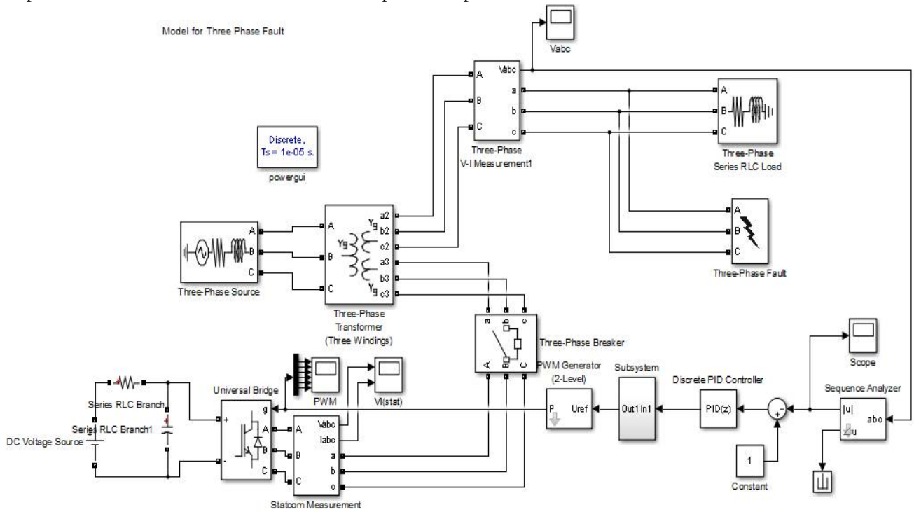
Fig 2 simulation model for three phase fault
